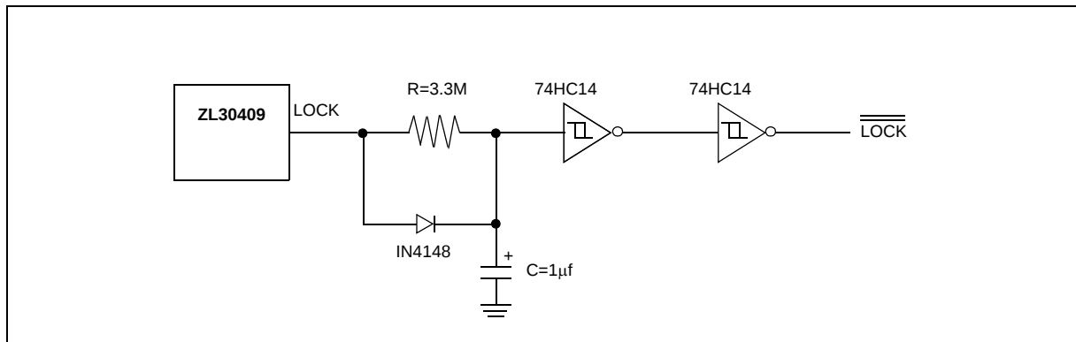
Figure 11 - Time-constant Circuit
