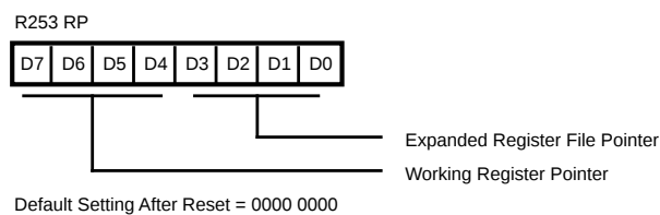
Figure 20. Register Pointer
