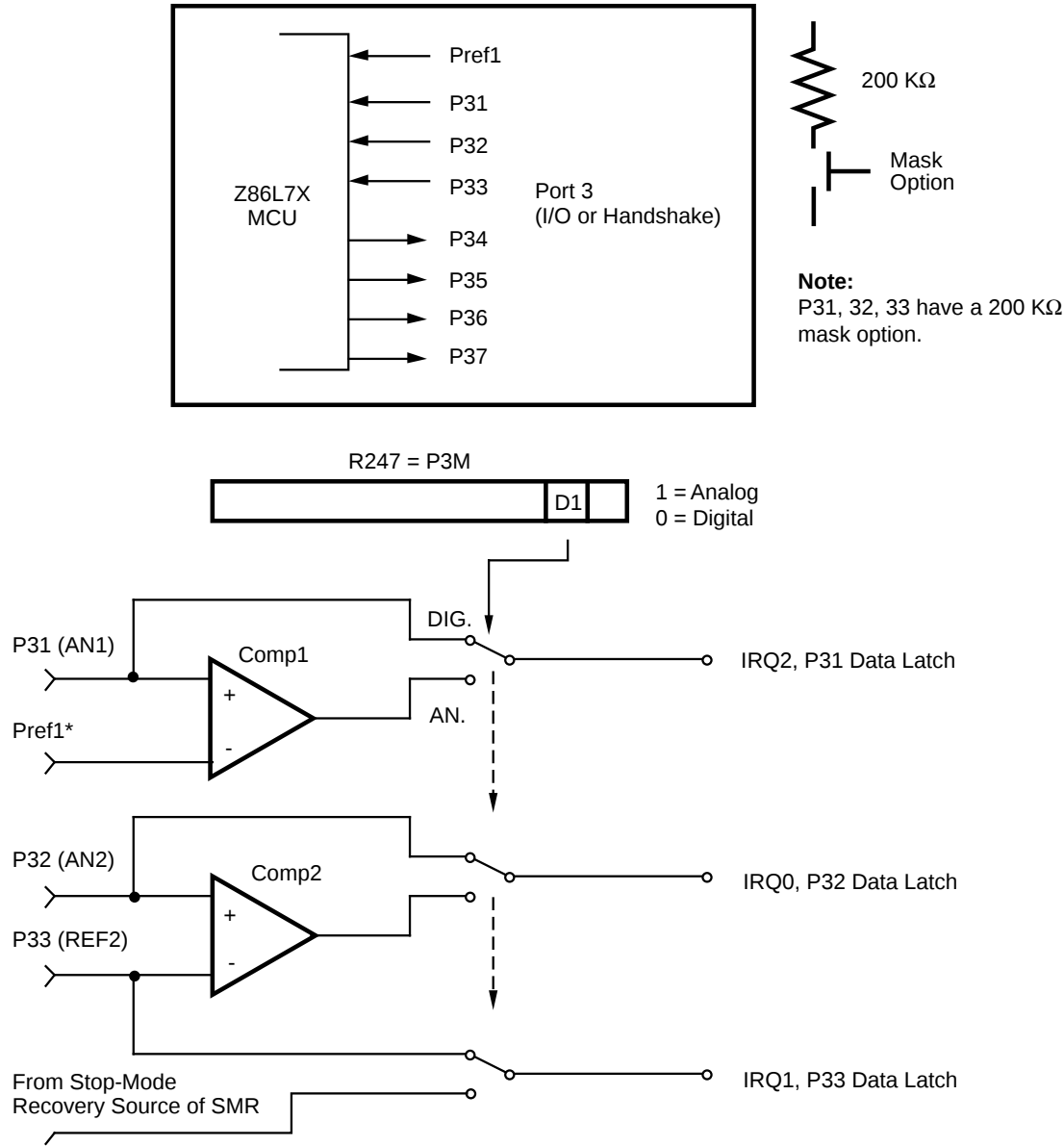
Figure 15. Port 3 Configuration
