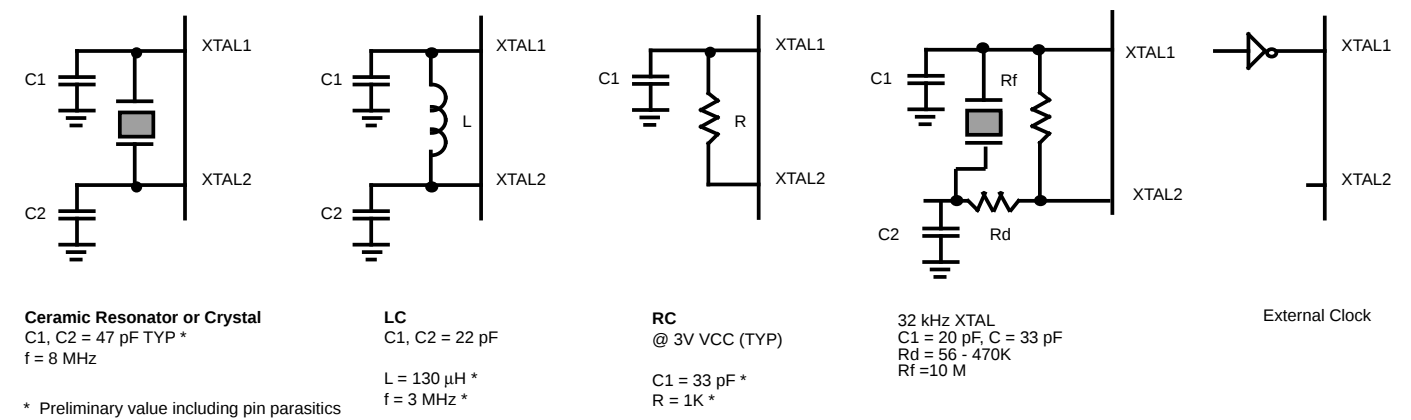
Figure 36. Oscillator Configuration
