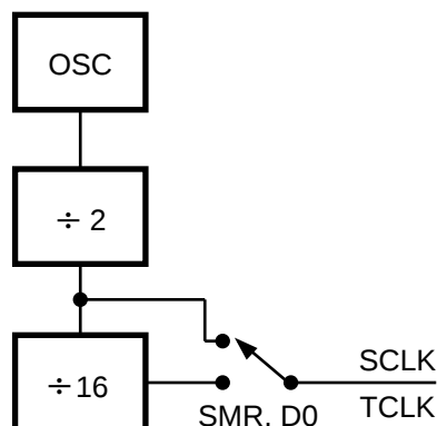
Figure 40. SCLK Circuit
