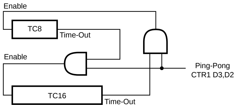
Figure 32. Ping-Pong Mode
