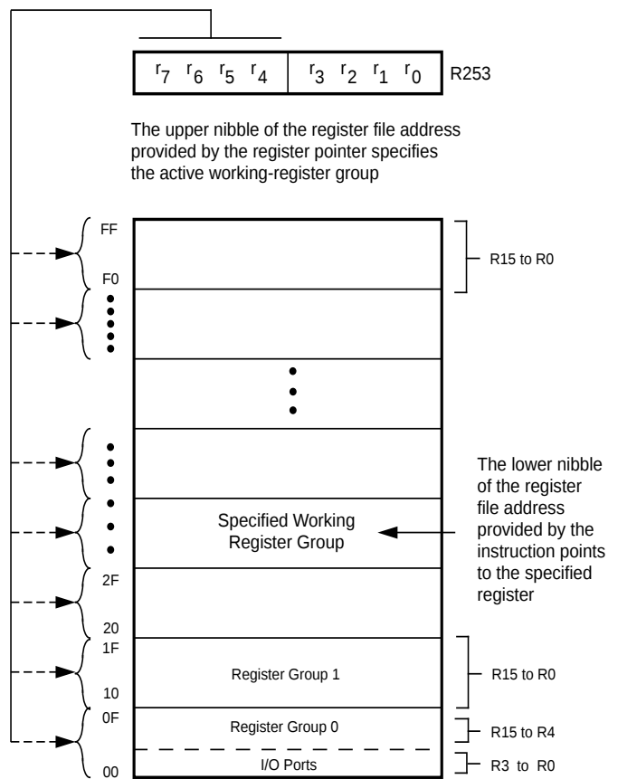
Figure 21. Register Pointer
