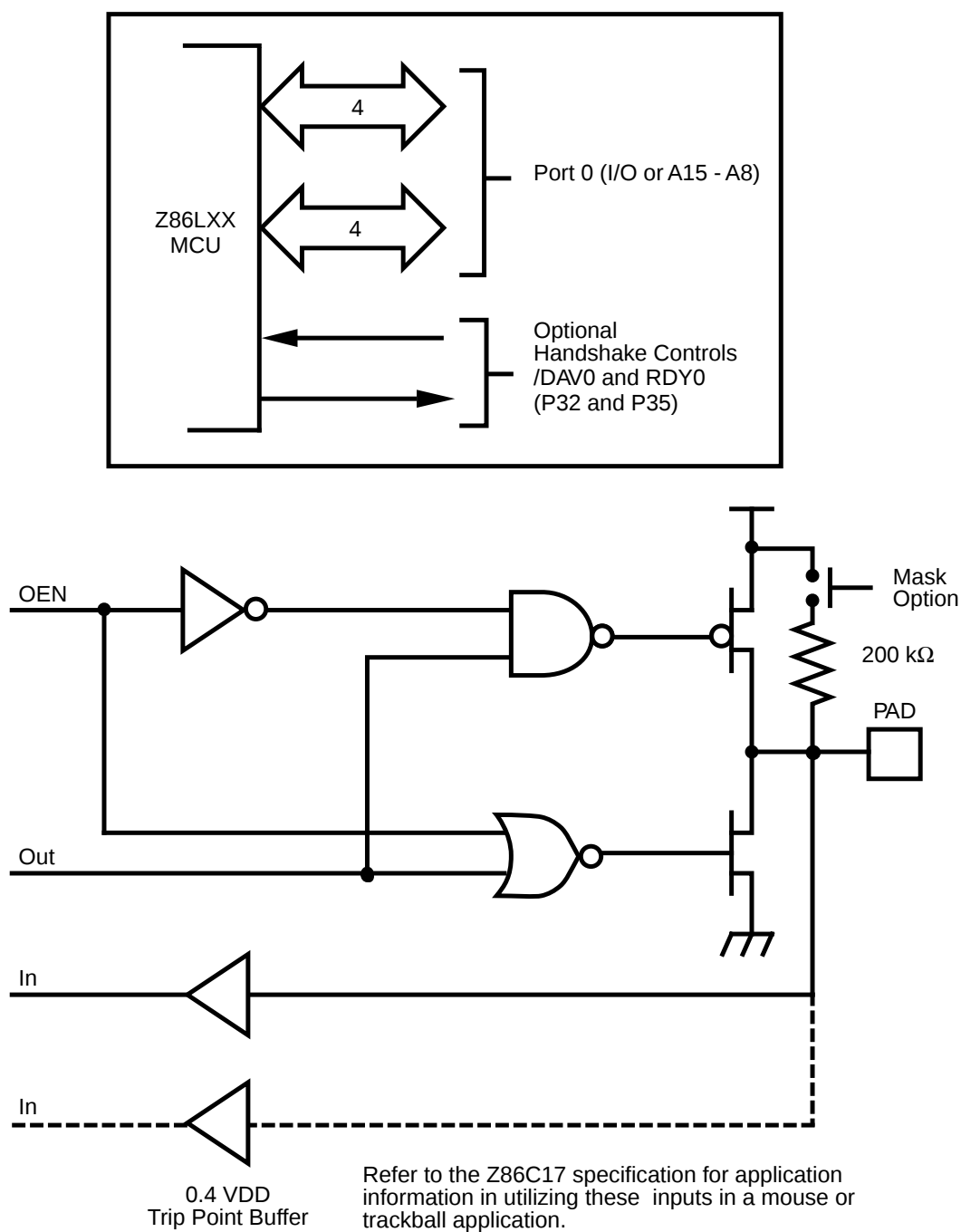
Figure 11. Port 0 Configuration
