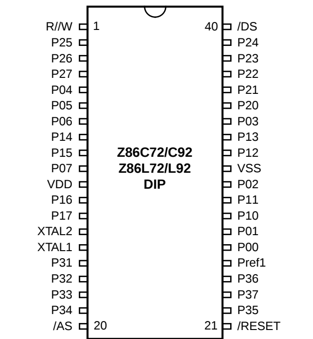
Figure 3. 40-Pin DIP Pin Assignments
